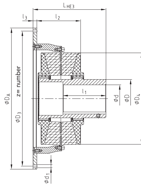
Flange dimensions acc. to SAE J 620 [mm]
