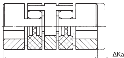
Axial displacement
