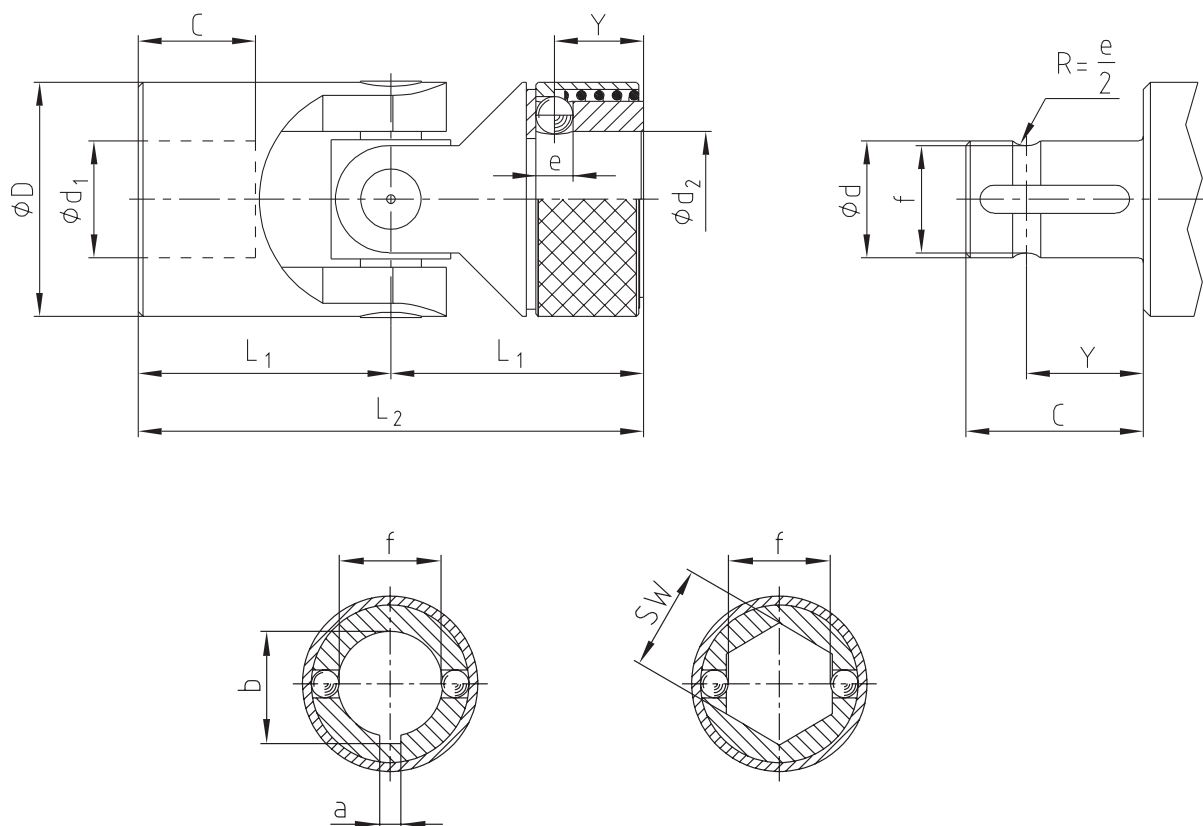
Type GR with plain bearing n_{max.} = 1000 rpm and type HR with needle bearing n_{max.} = 4000 rpm
