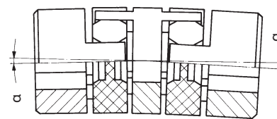
Angular displacement
