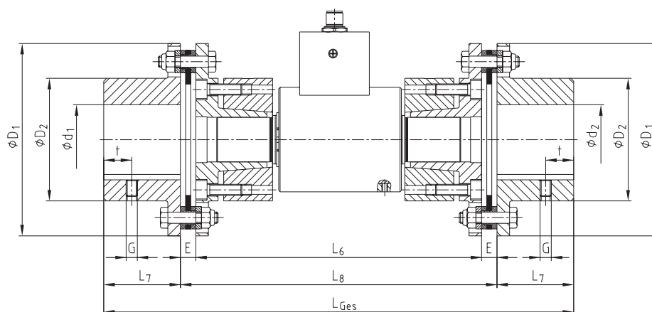
Combination of DATAFLEX® 32 with RADEX®-N
