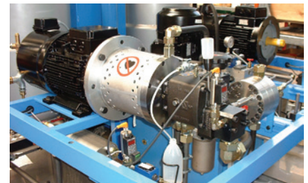
Maintenance-free sealing of dosing pumps for polyol and isocyanate in high-pressure reaction casting machines
