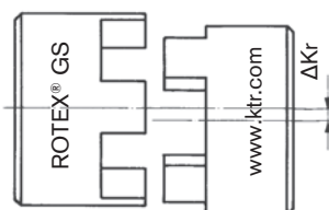
Radial displacement
