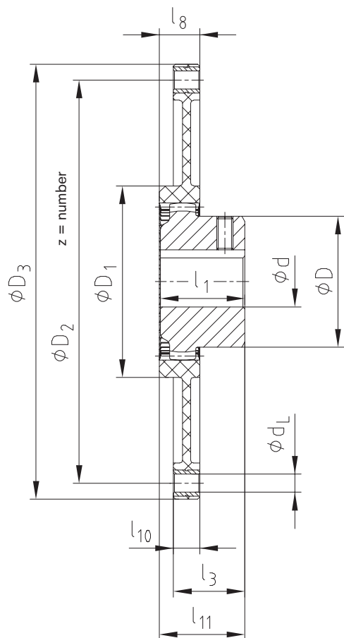
Short mounting
