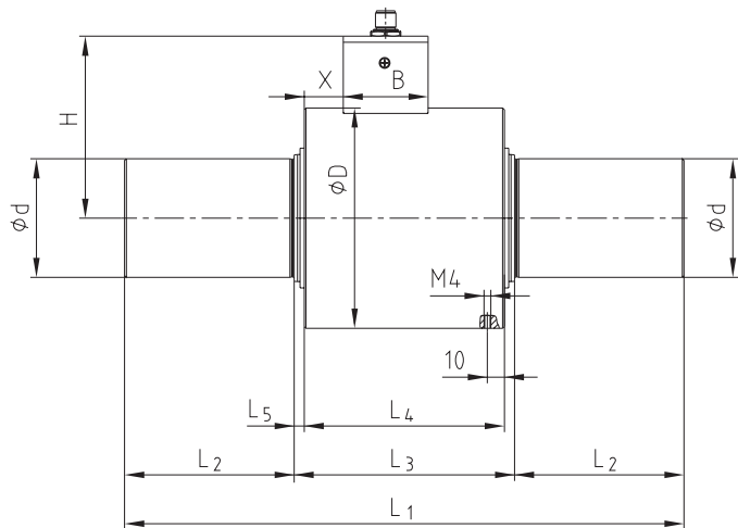
Combination of DATAFLEX® 70 with RADEX®-N
