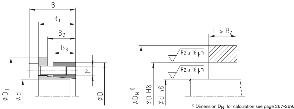
Example of application of hub type
