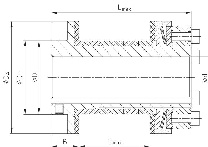
Technical data – Dimensions
