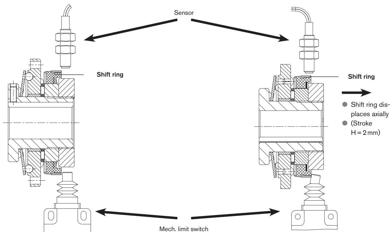
Signal by limit switch or sensor in case of overload
