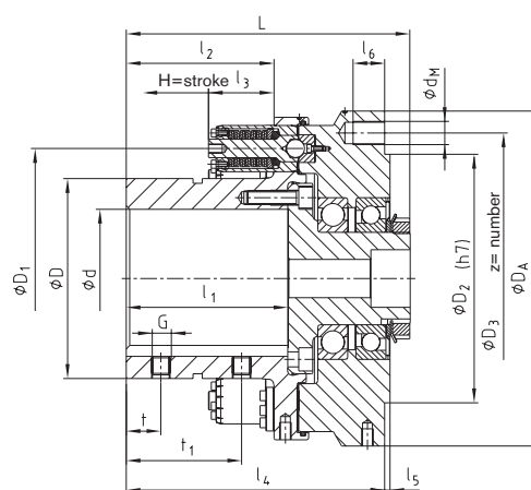
Torques [Nm]
