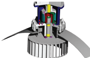
MINEX ® -S for sealing of autoclaves (T.B.M. / STERICHEM) in laboratories and hospitals
